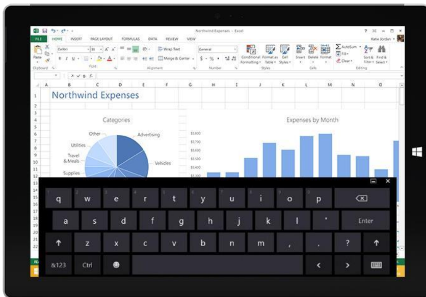
On-screen keyboard
